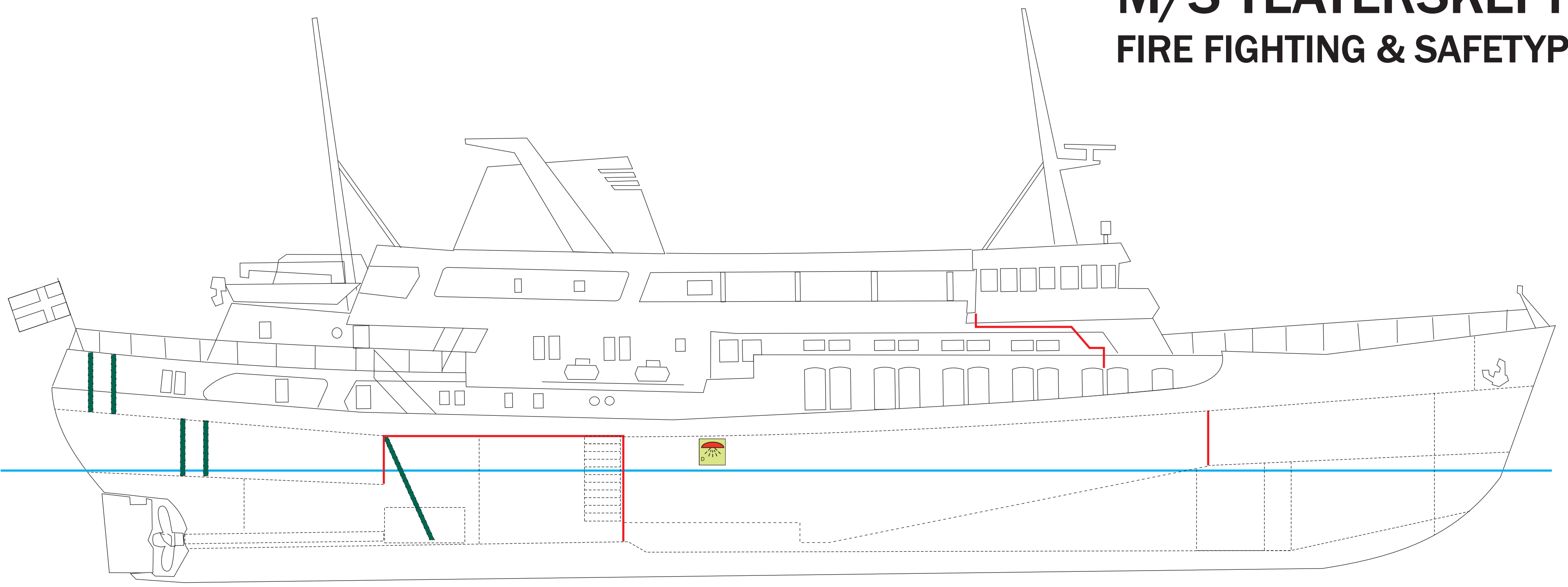
BRIDGE DECK
